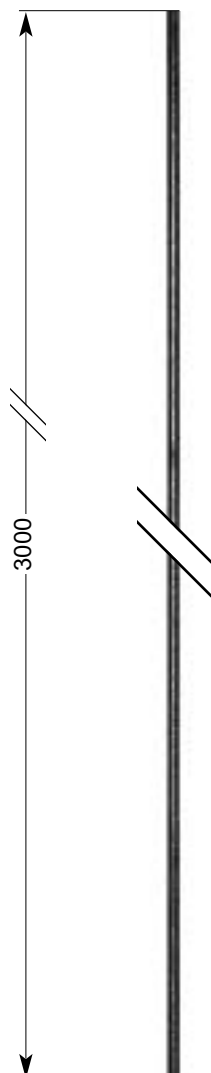
12 114 Rundmaterial Roundmaterial Matériau ronde 1,21 kg / m L. 3 m Ø 14 mm
